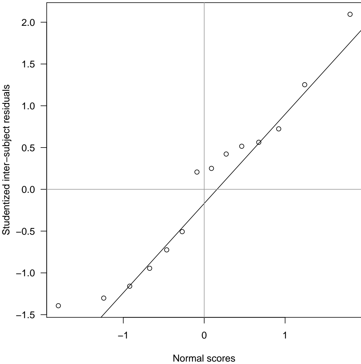
Normal Probability Plot of InCmax (intersubj)
